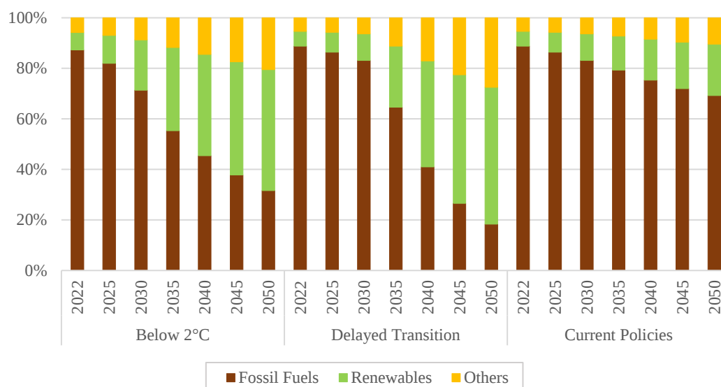
Chart 6: Primary energy mix 5 in Mainland China under the long-term scenarios
